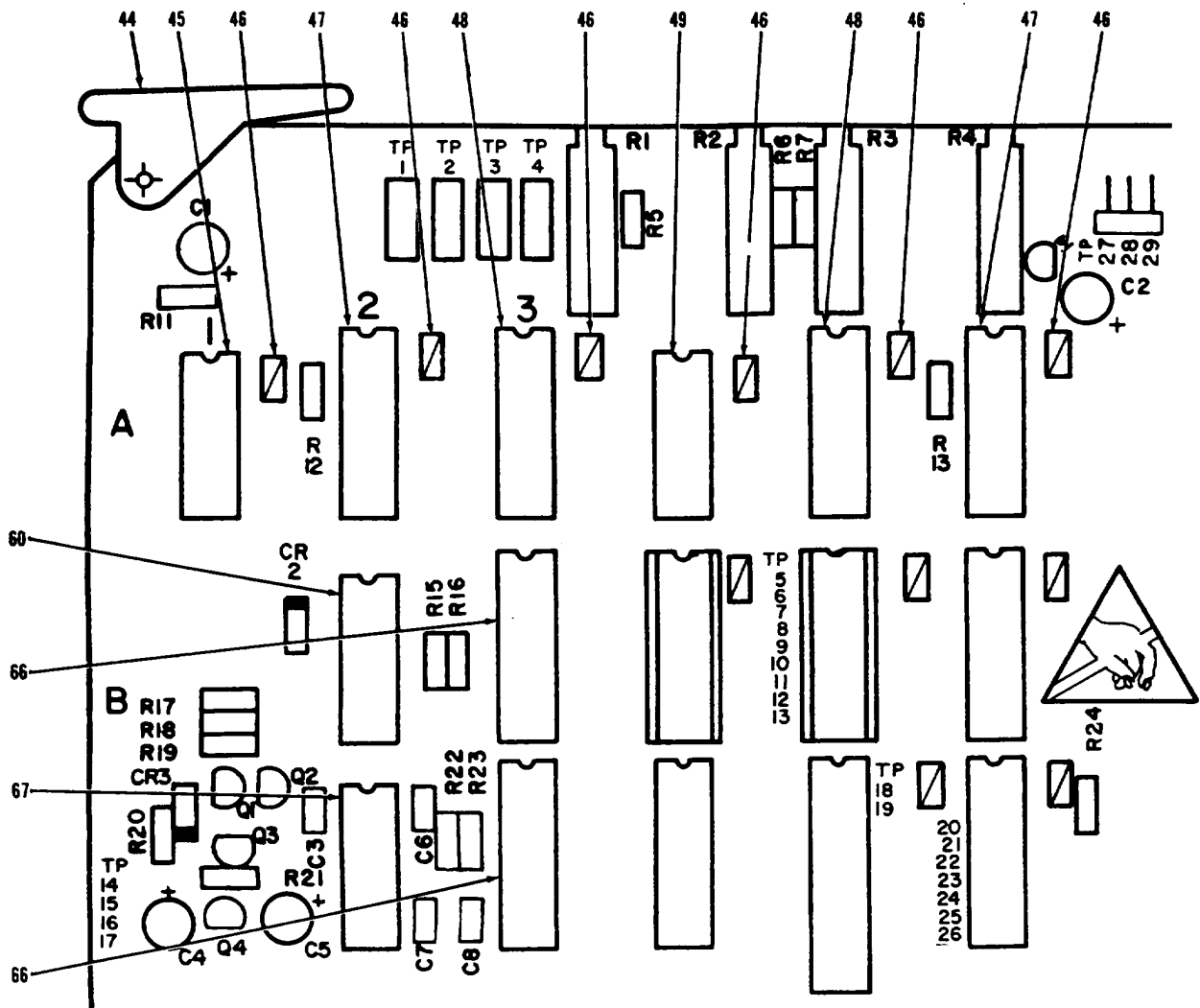
Figure 17. Circuit Card Assembly, Reference 2703 (Sheet 1 of 9)
