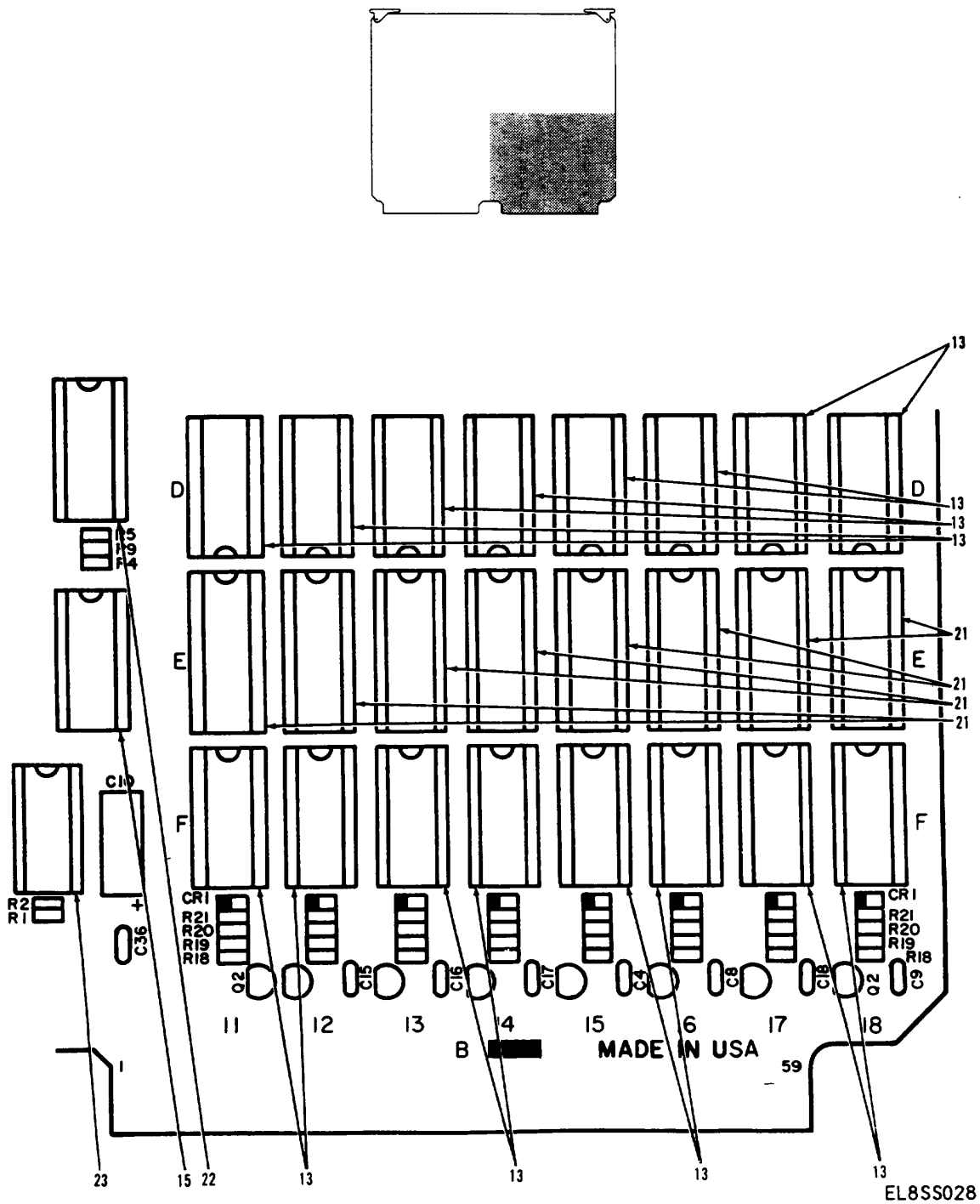
Figure 12. Circuit Card Assembly, Driver Sensor (Sheet 3 of 9)
