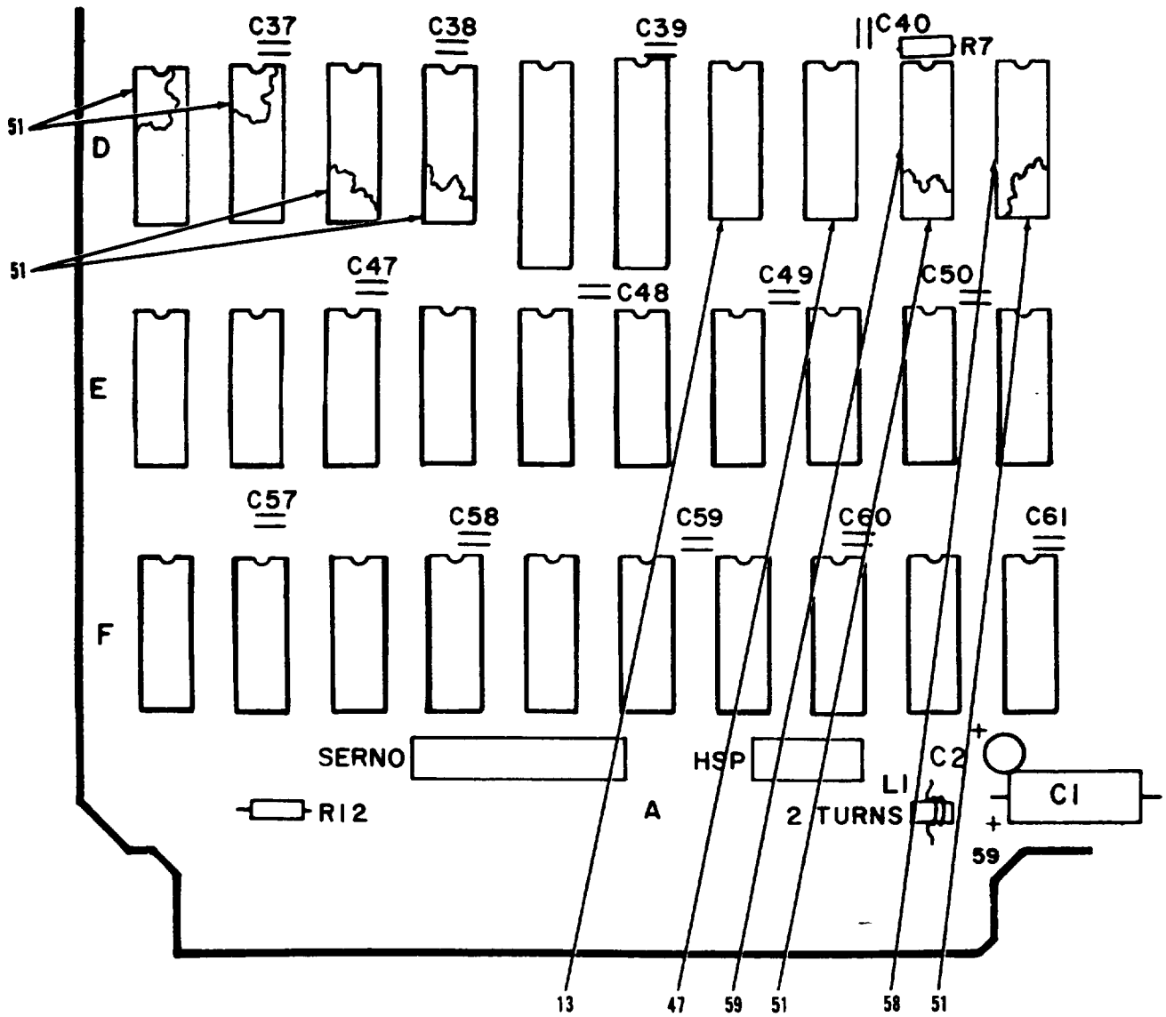
Figure 13. Circuit Card Assembly, Pin Processor (Sheet 8 of 9)
