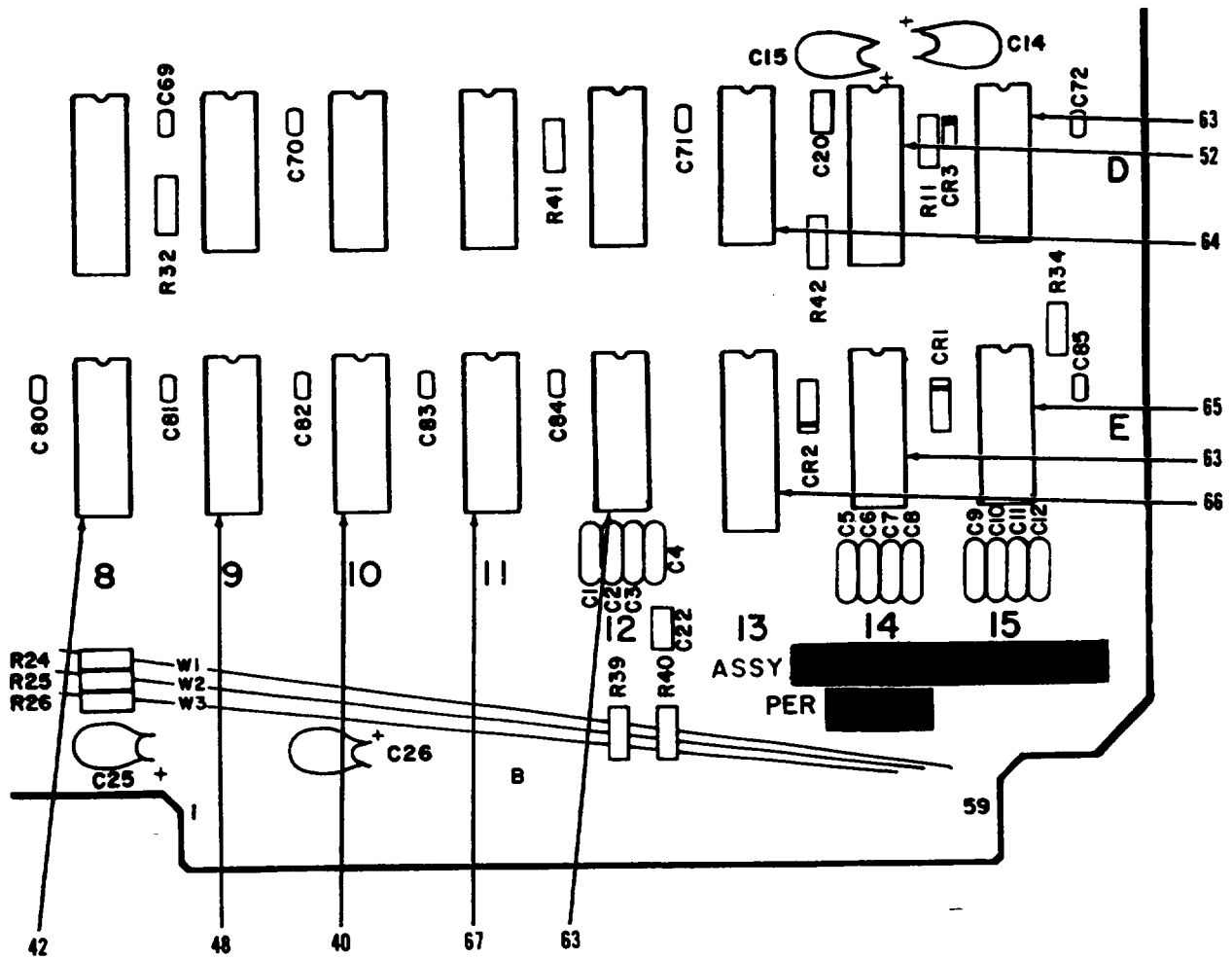
Figure 15. Circuit Card Assembly, Peripheral (Sheet 3 of 9)
