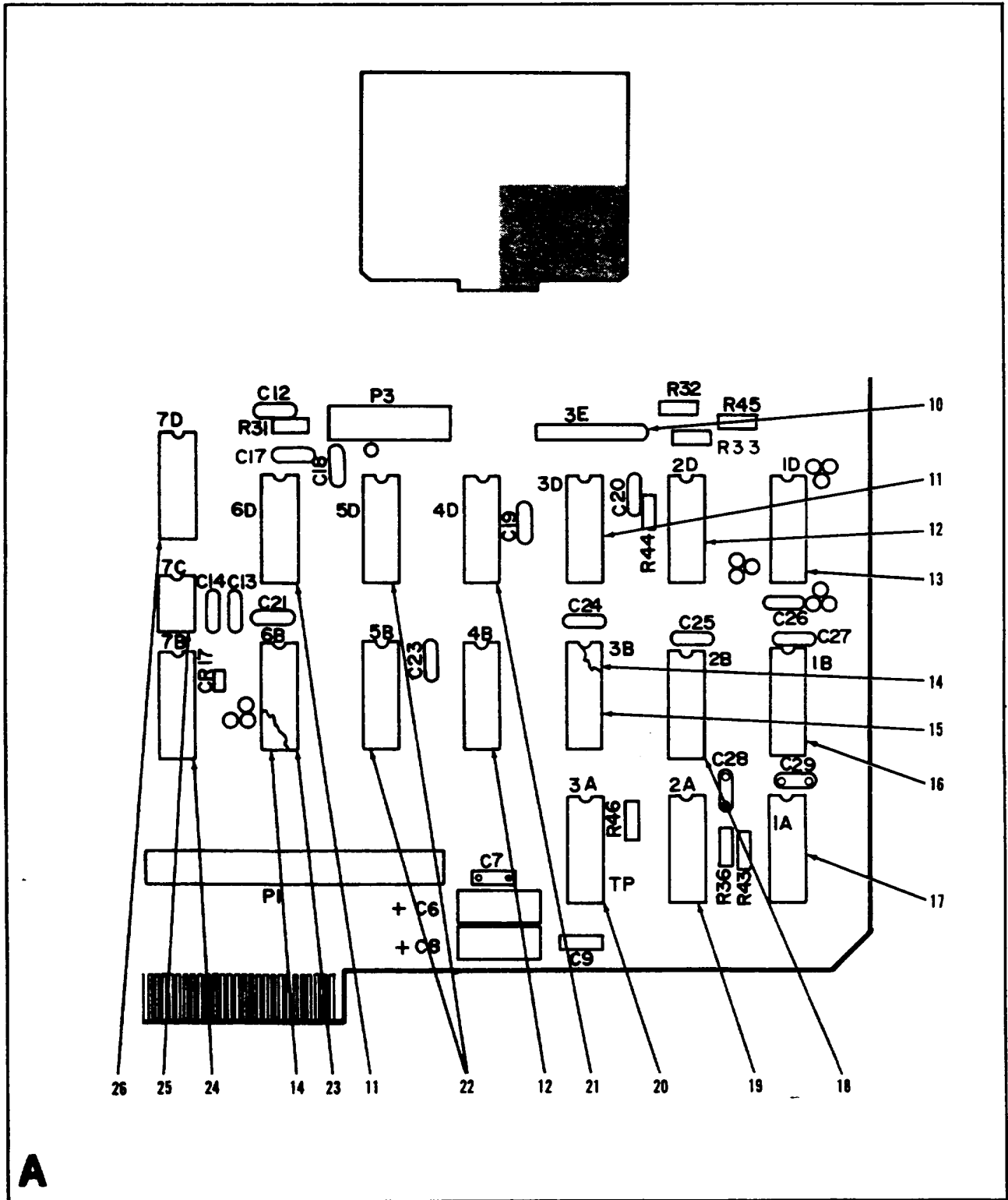
Figure 10. Circuit Card Assembly, Keyboard (Sheet 3 of 5)
