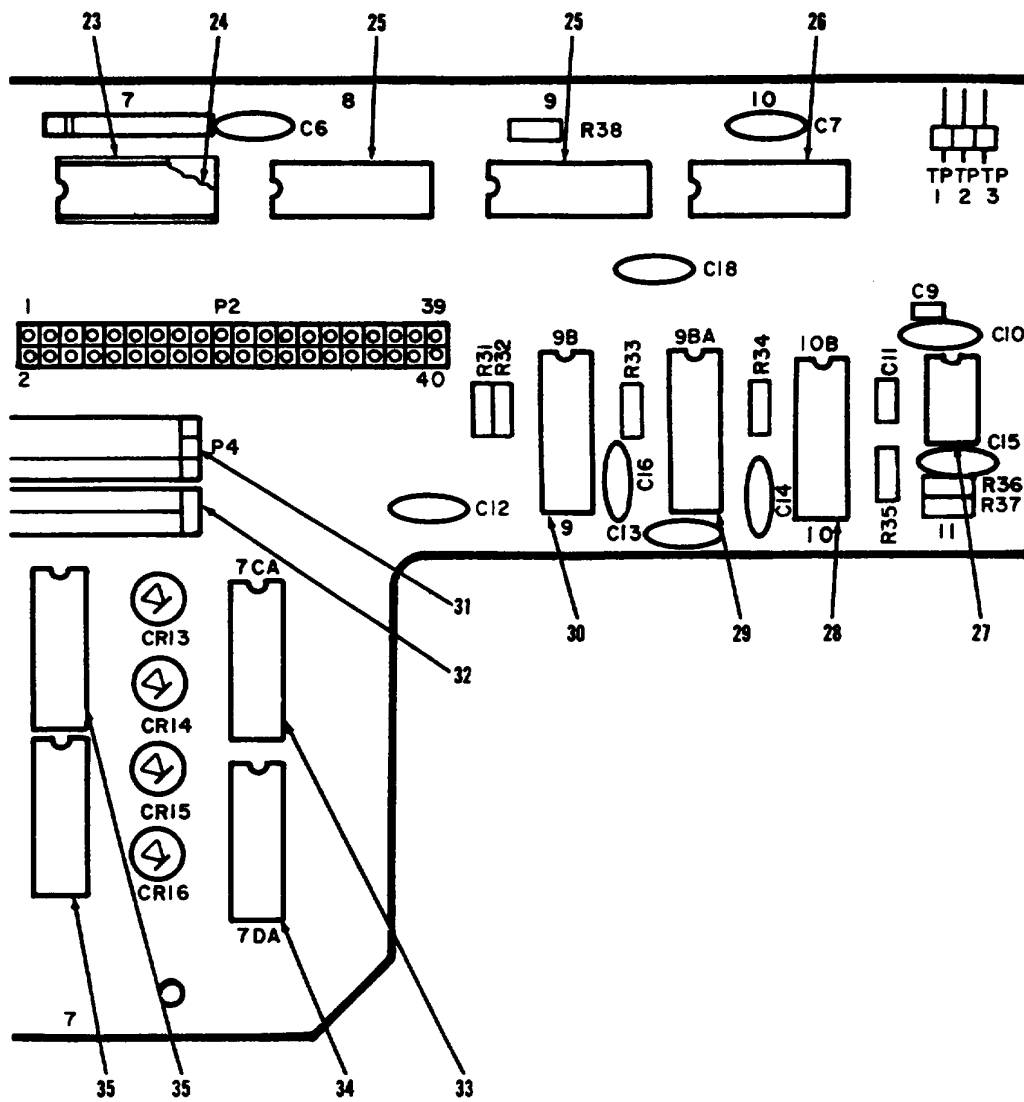
Figure 11. Circuit Card Assembly, Display (Sheet 2 of 3)
