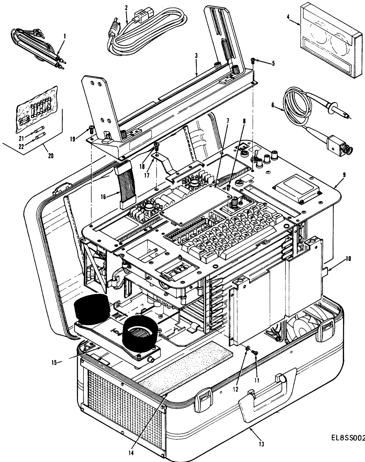
Figure 2. Digital Card Tester
