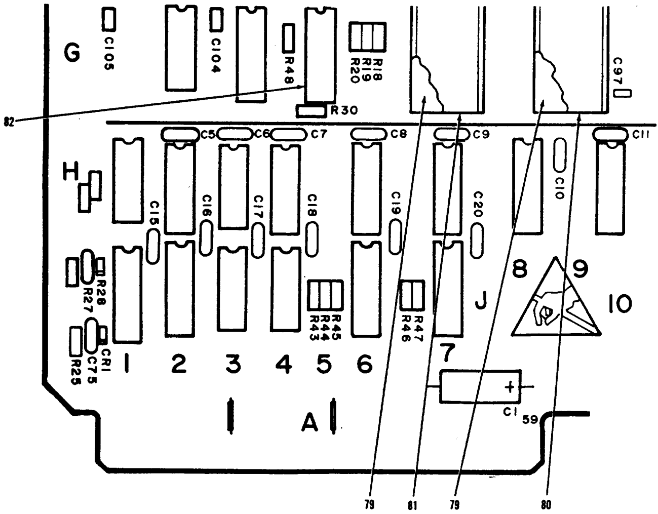
Figure 14. Circuit Card Assembly, Processor (Sheet 8 of 9)
