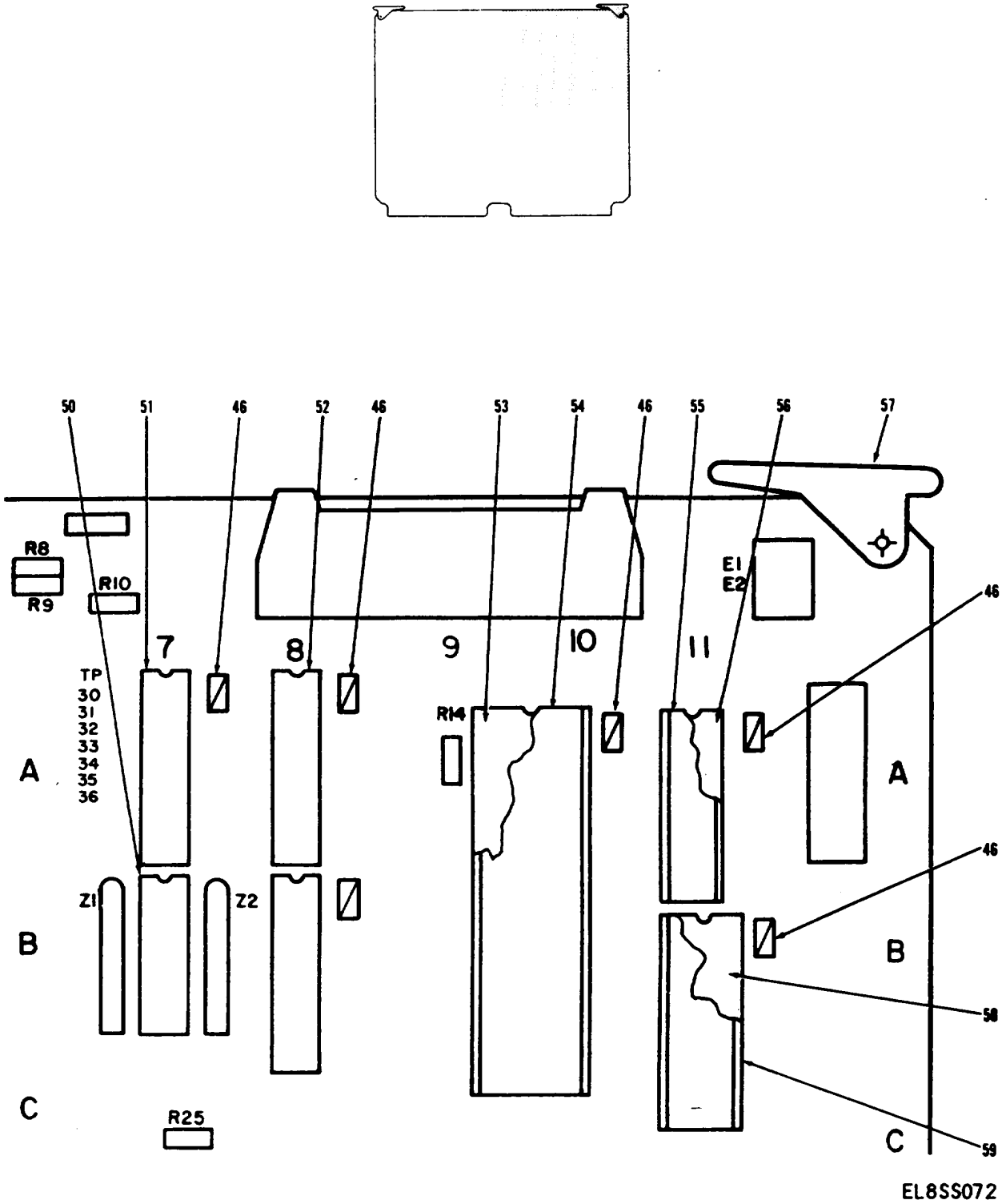
Figure 17. Circuit Card Assembly, Reference 2703 (Sheet 2 of 9)
