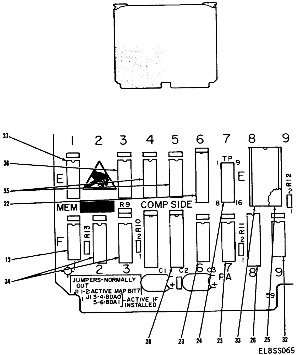
Figure 16. Circuit Card Assembly, 512K Memory (Sheet 4 of 5)
