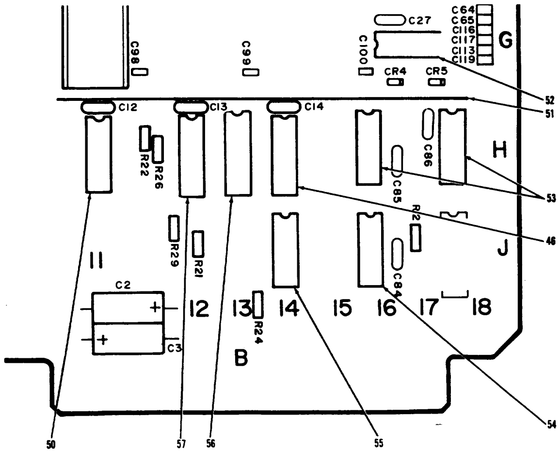
Figure 14. Circuit Card Assembly, Processor (Sheet 3 of 9)
