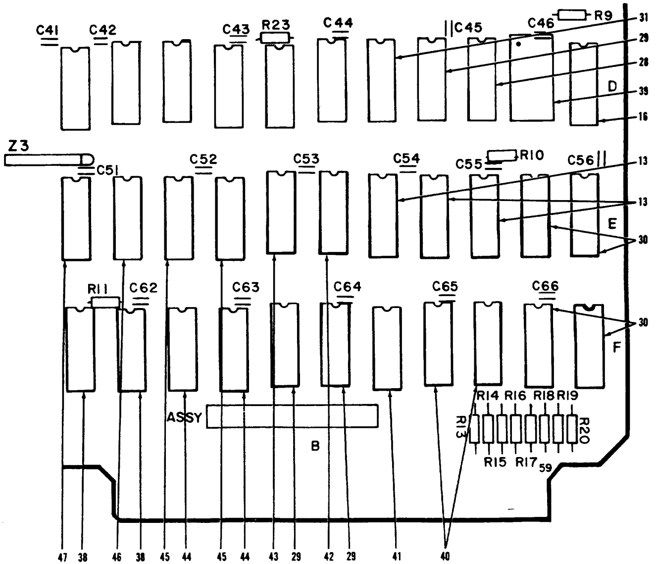
Figure 13. Circuit Card Assembly, Pin Processor (Sheet 3 of 9)
