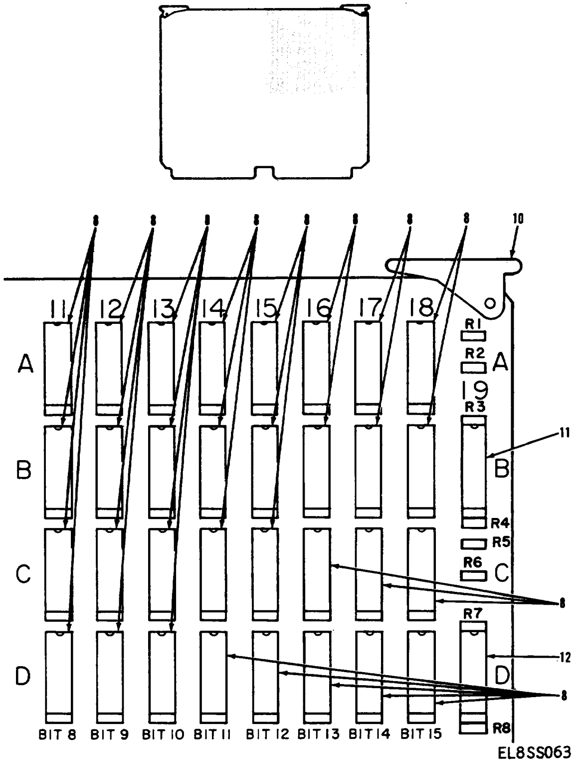
Figure 16. Circuit Card Assembly, 512K Memory (Sheet 2 of 5)
