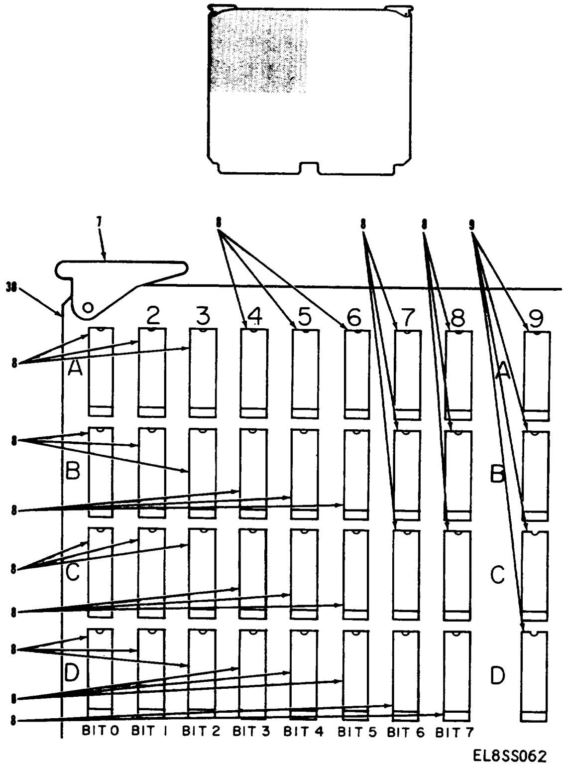
Figure 16. Circuit Card Assembly, 512K Memory (Sheet 1 of 5)
