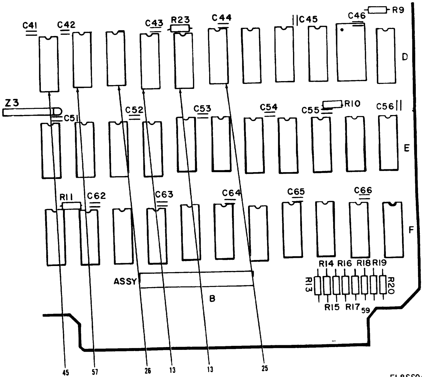
Figure 13. Circuit Card Assembly, Pin Processor (Sheet 7 of 9)
