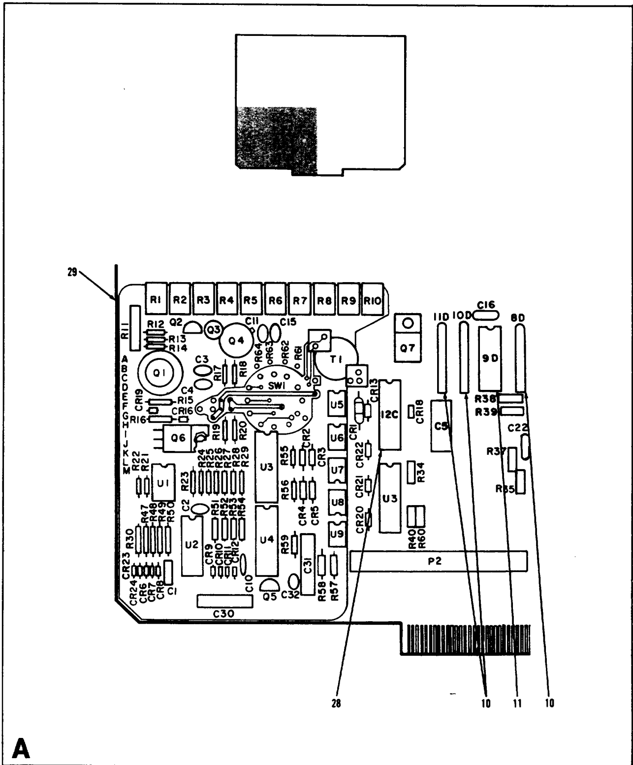
Figure 10. Circuit Card Assembly, Keyboard (Sheet 4 of 5)
