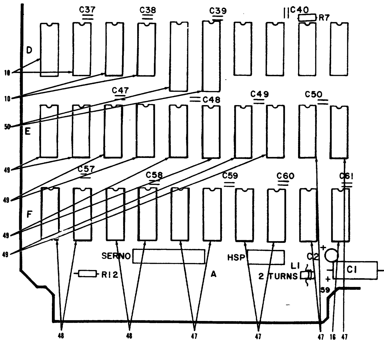
Figure 13. Circuit Card Assembly, Pin Processor (Sheet 4 of 9)
