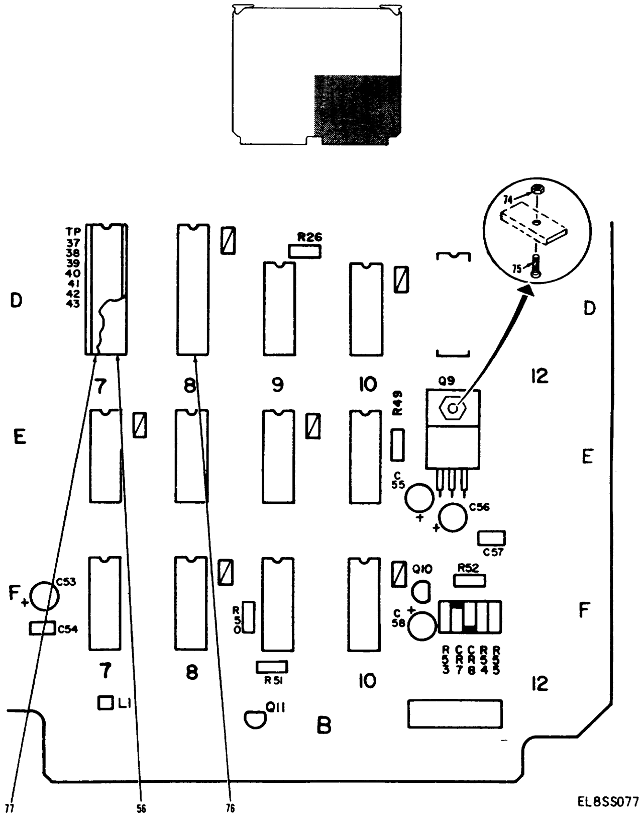
Figure 17. Circuit Card Assembly, Reference 2703 (Sheet 7 of 9)
