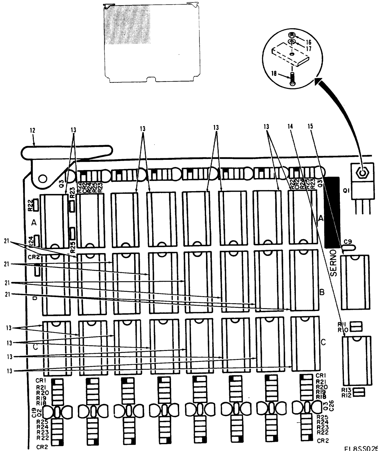
Figure 12. Circuit Card Assembly, Driver Sensor (Sheet 1 of 9)
