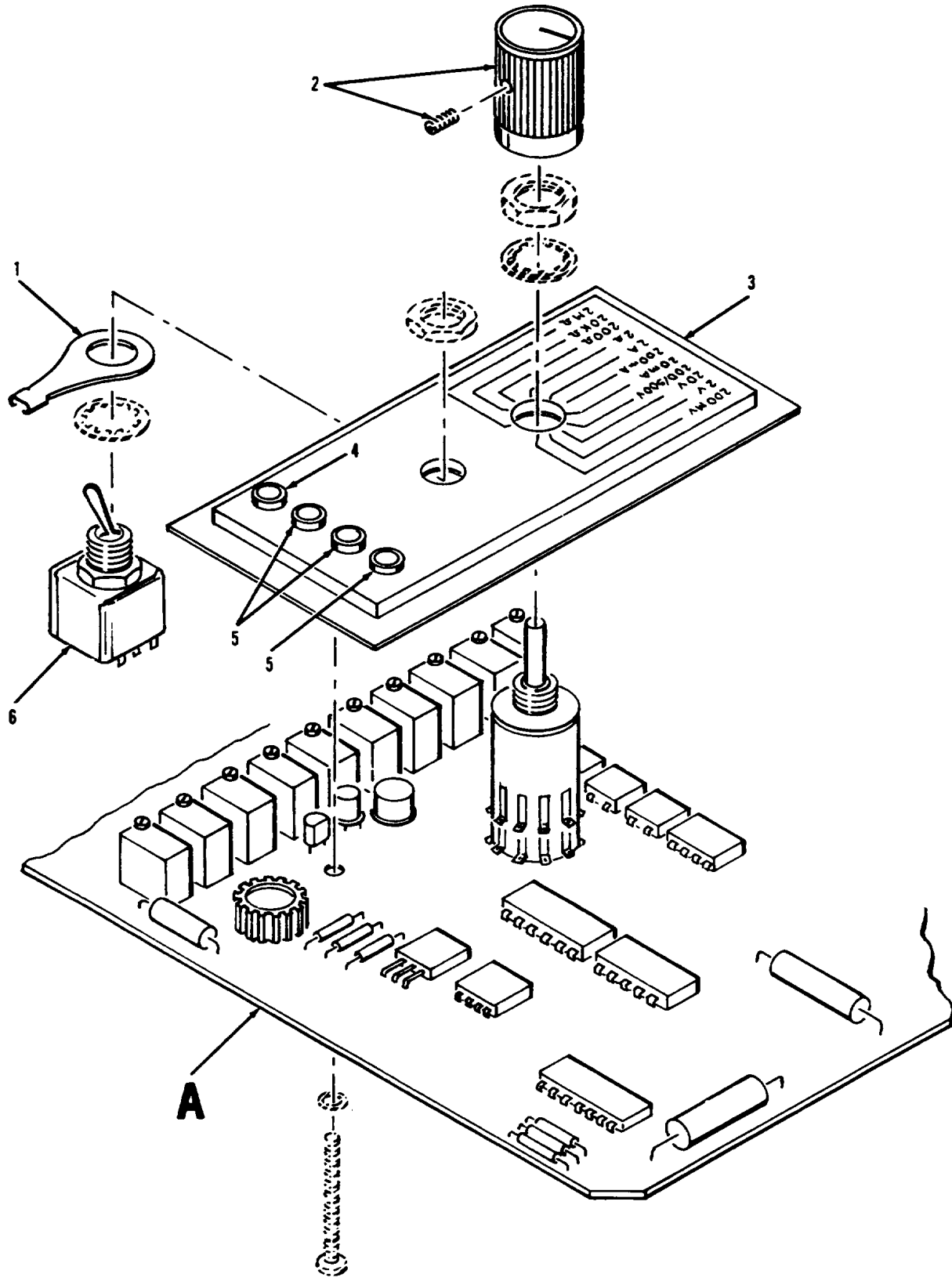
Figure 10. Circuit Card Assembly, Keyboard (Sheet 1 of 5)
