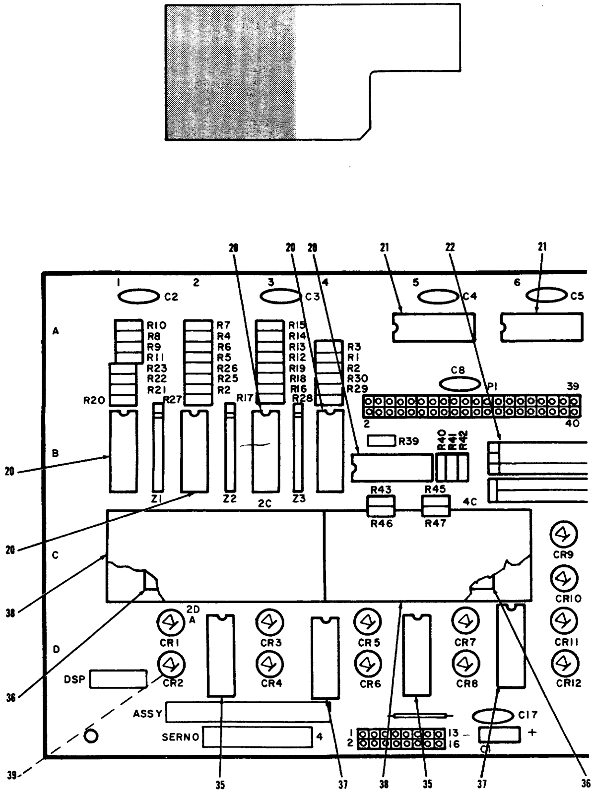
Figure 11. Circuit Card Assembly, Display (Sheet 1 of 3)
