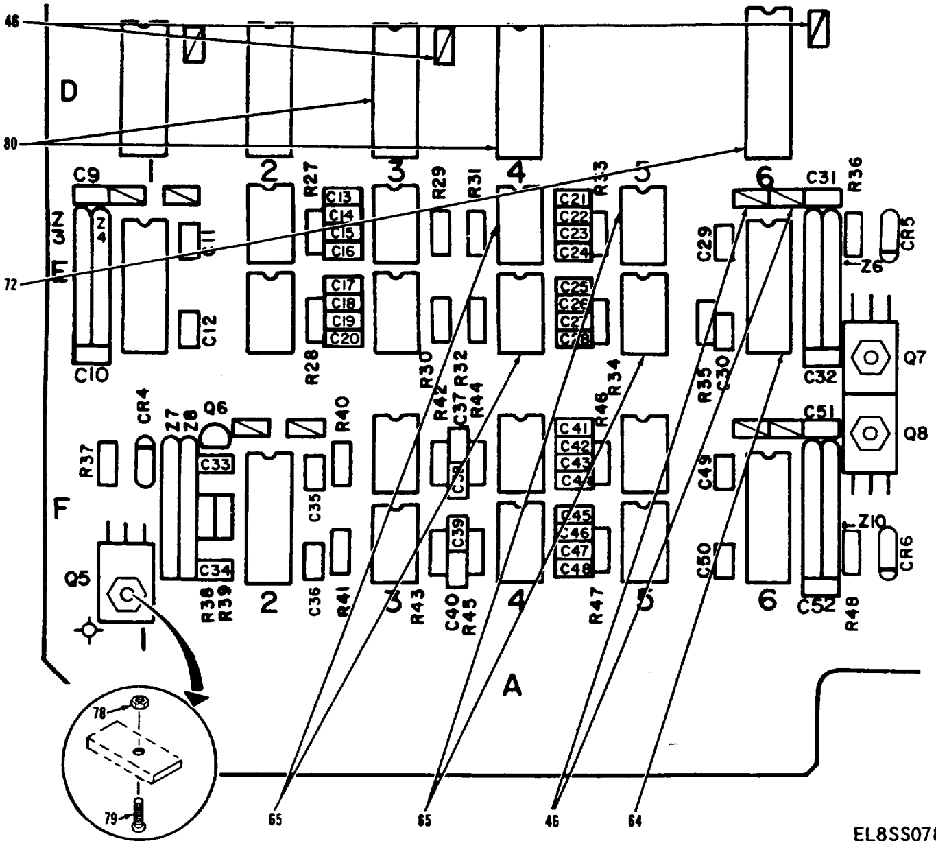
Figure 17. Circuit Card Assembly, Reference 2703 (Sheet 8 of 9)
