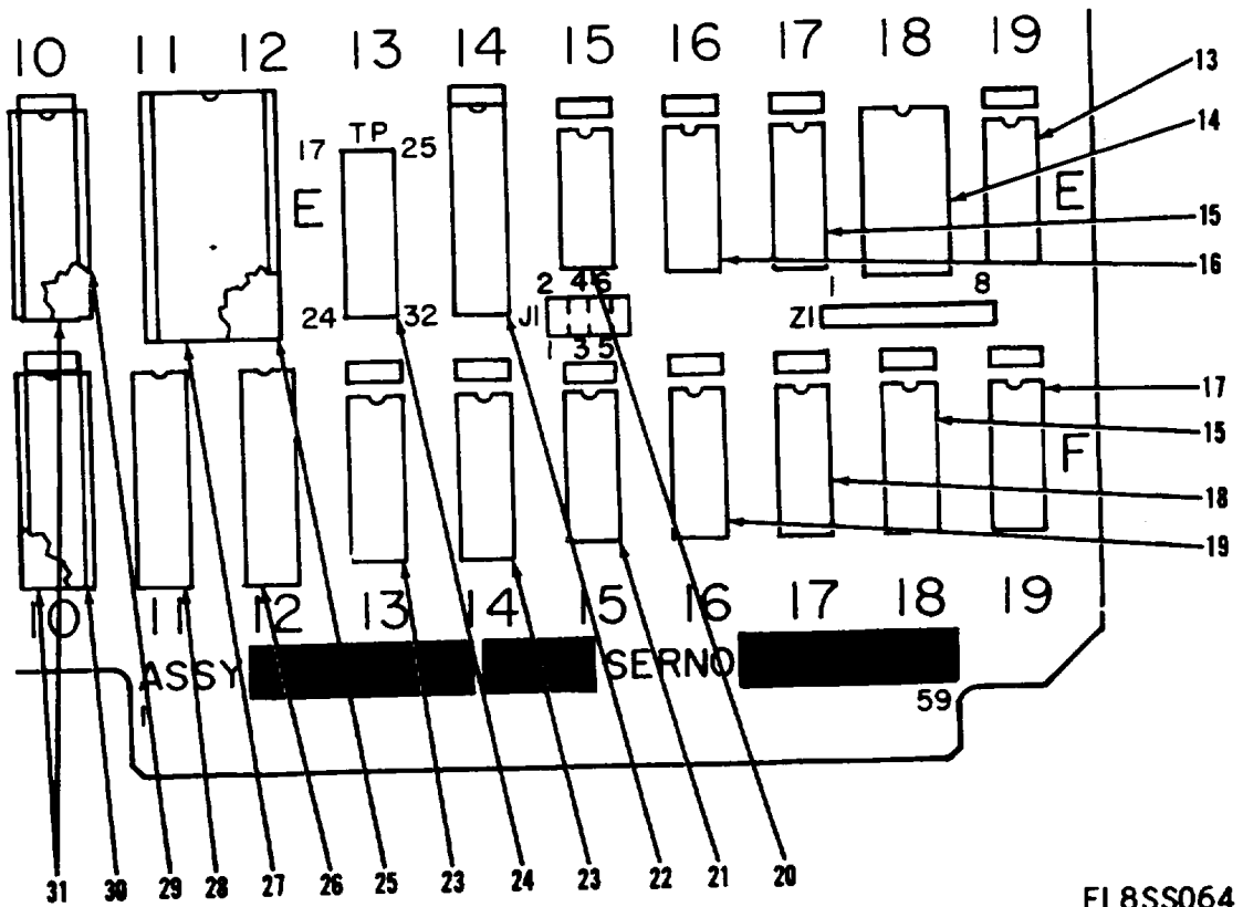
Figure 16. Circuit Card Assembly, 512K Memory (Sheet 3 of 5)
