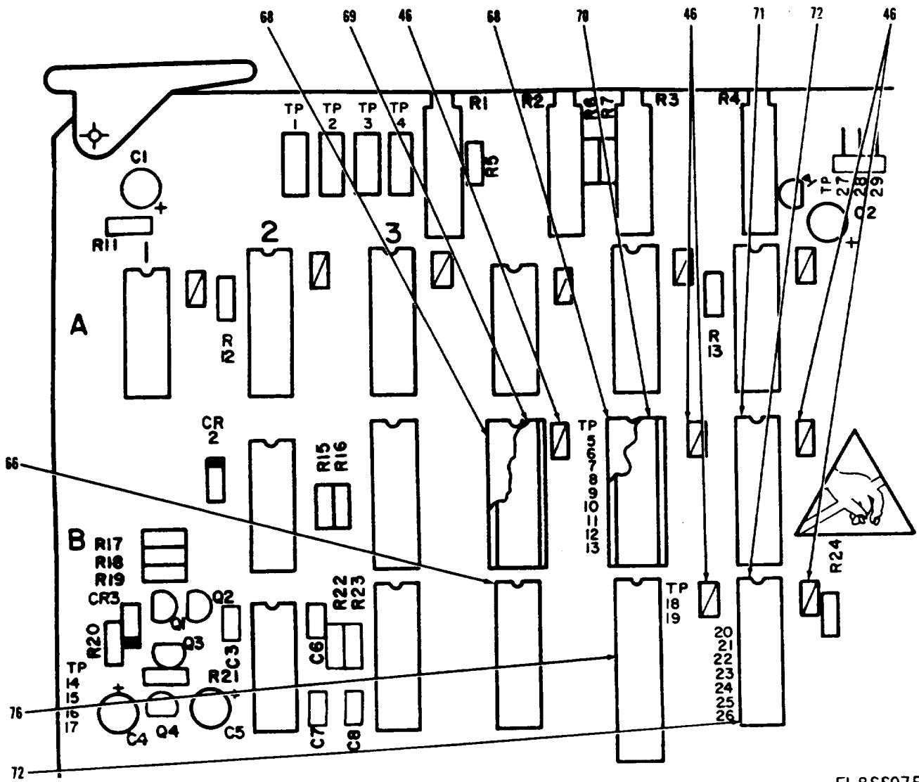
Figure 17. Circuit Card Assembly, Reference 2703 (Sheet 5 of 9)
