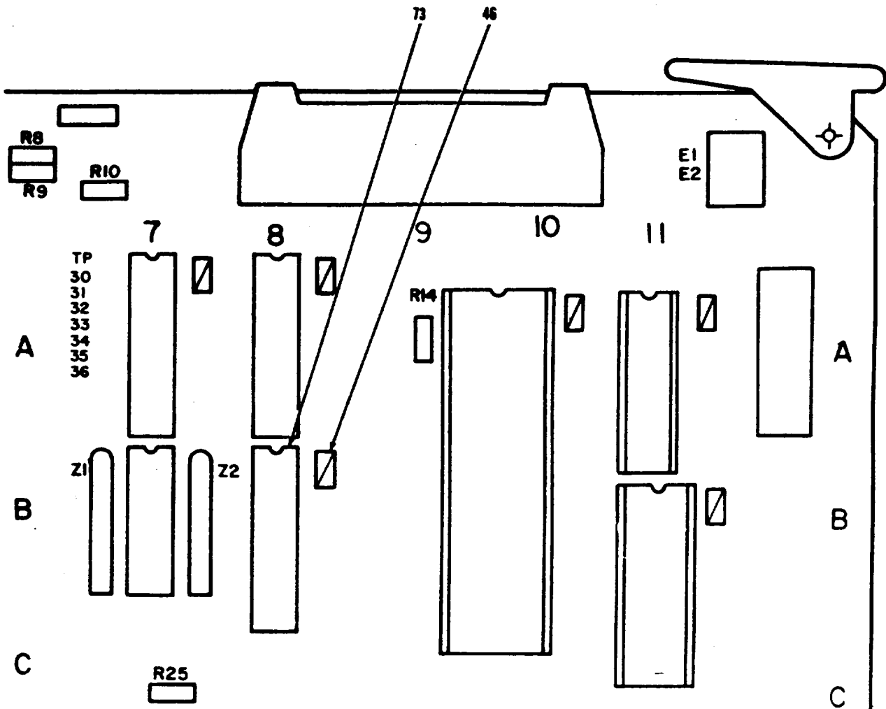
Figure 17. Circuit Card Assembly, Reference 2703 (Sheet 6 of 9)
