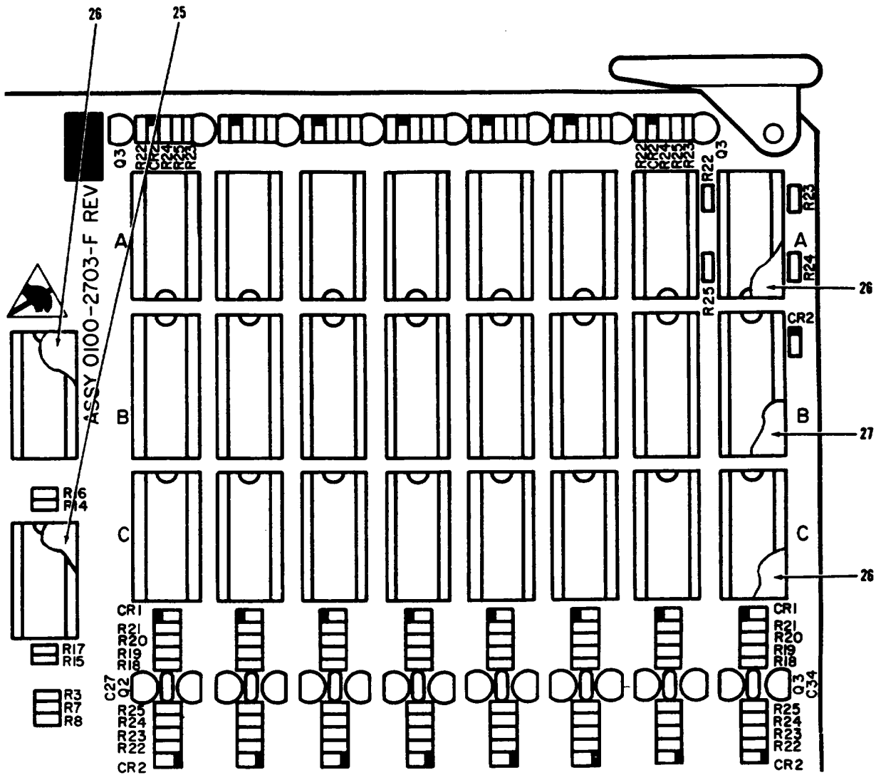
Figure 12. Circuit Card Assembly, Driver Sensor (Sheet 6 of 9)
