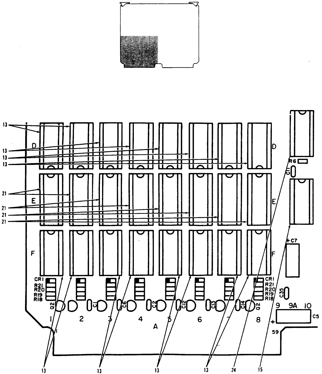
Figure 12. Circuit Card Assembly, Driver Sensor (Sheet 4 of 9)
