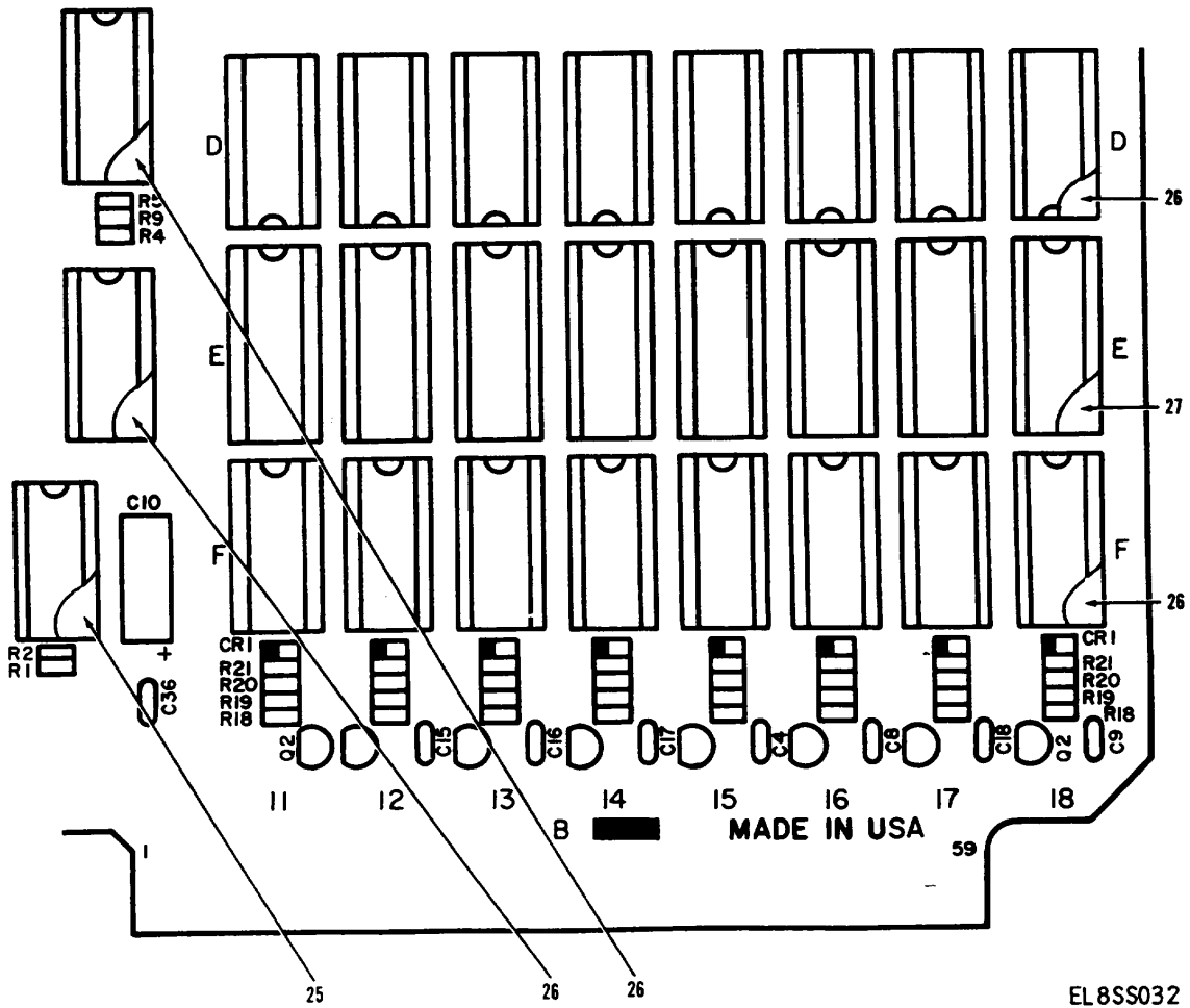
Figure 12. Circuit Card Assembly, Driver Sensor (Sheet 7 of 9)
