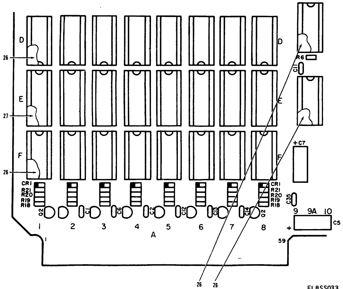
Figure 12. Circuit Card Assembly, Driver Sensor (Sheet 8 of 9)
