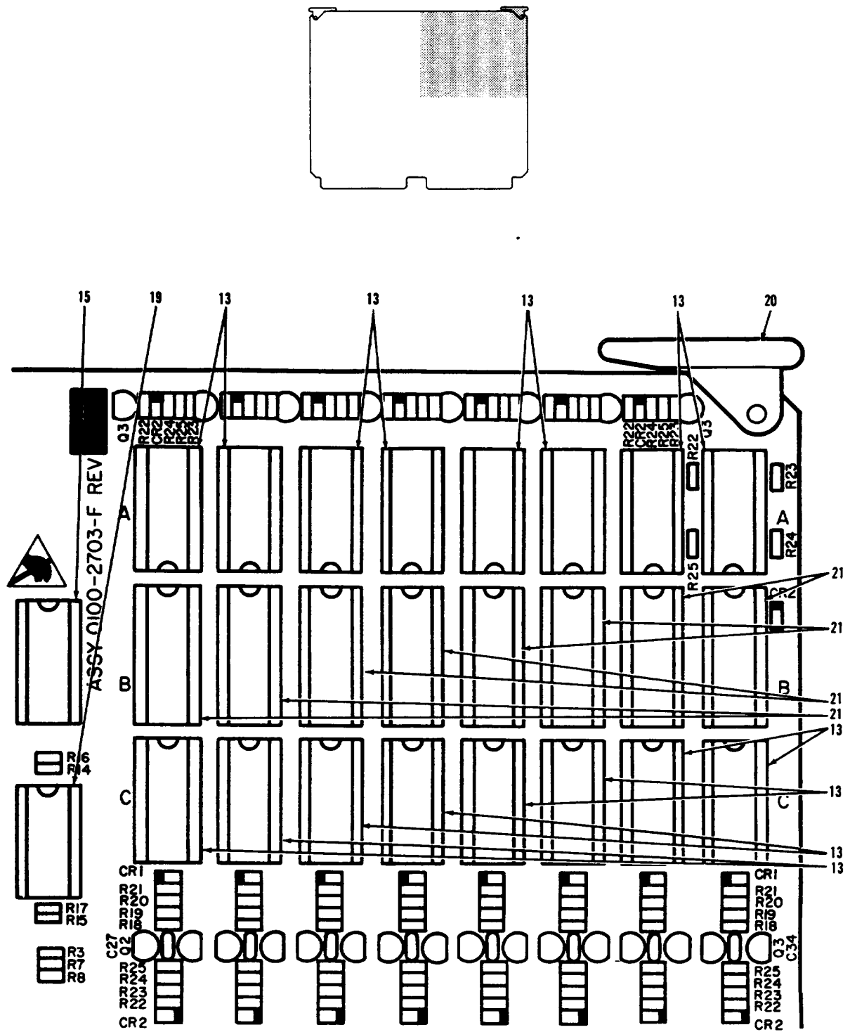
Figure 12. Circuit Card Assembly, Driver Sensor (Sheet 2 of 9)
