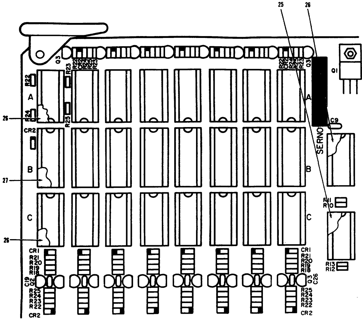
Figure 12. Circuit Card Assembly, Driver Sensor (Sheet 5 of 9)
