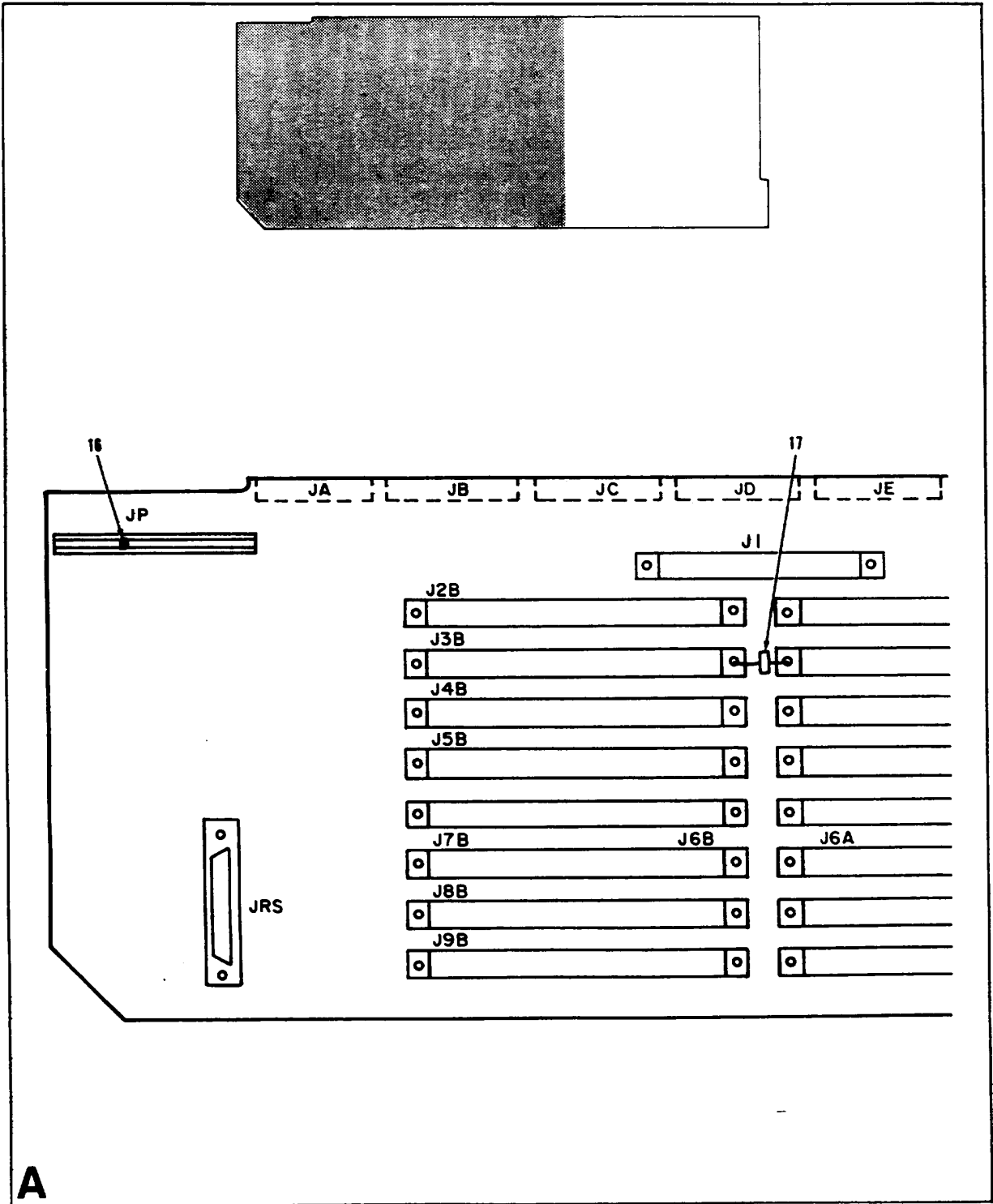
Figure 6. Motherboard Assembly (Sheet 2 of 4)
