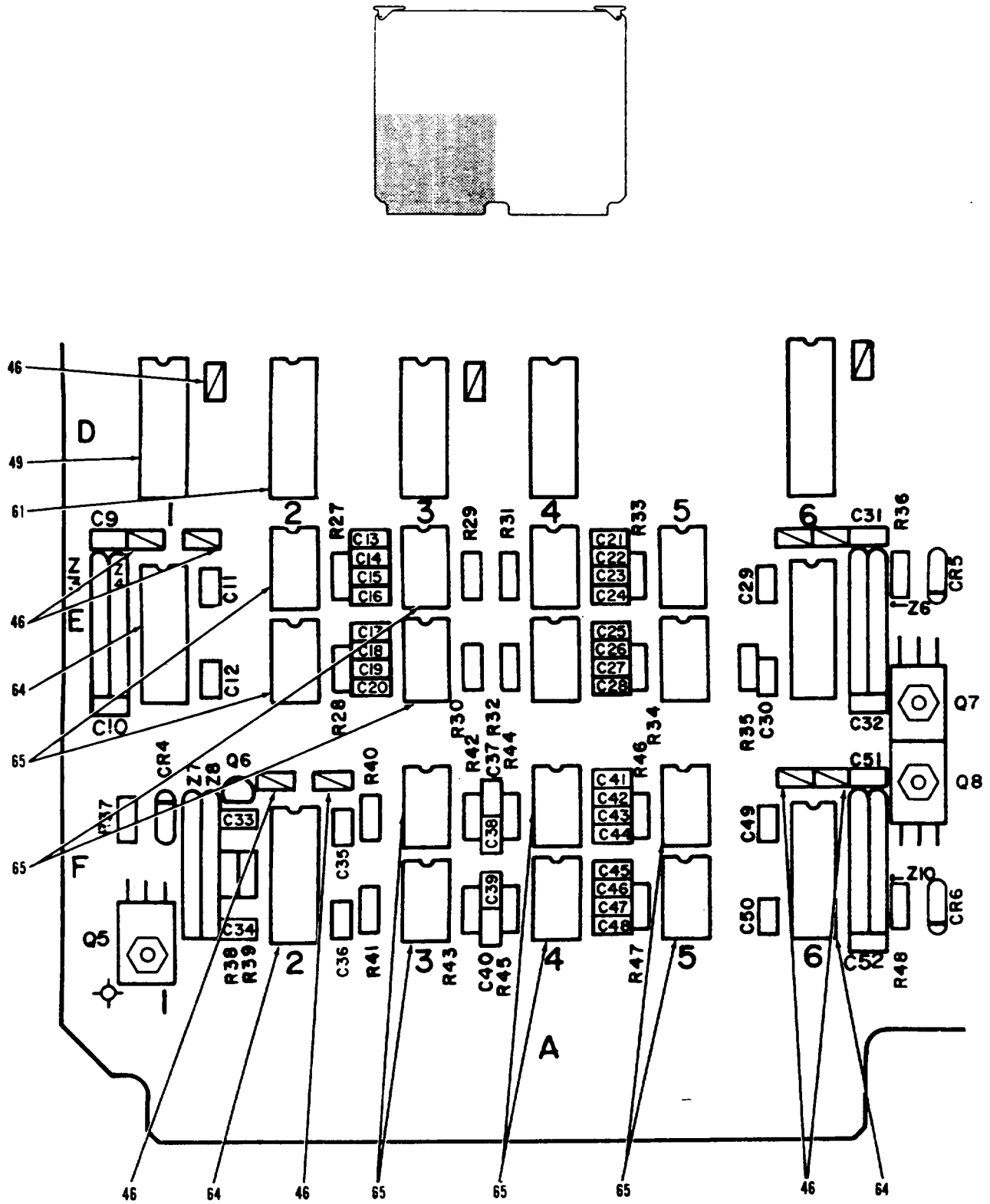
Figure 17. Circuit Card Assembly, Reference 2703 (Sheet 4 of 9)
