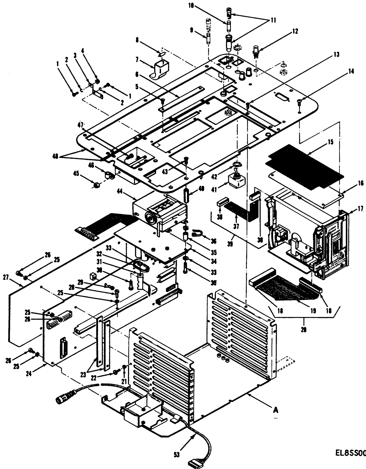
Figure 4. Card Cage Assembly (Sheet 1 of 2)
