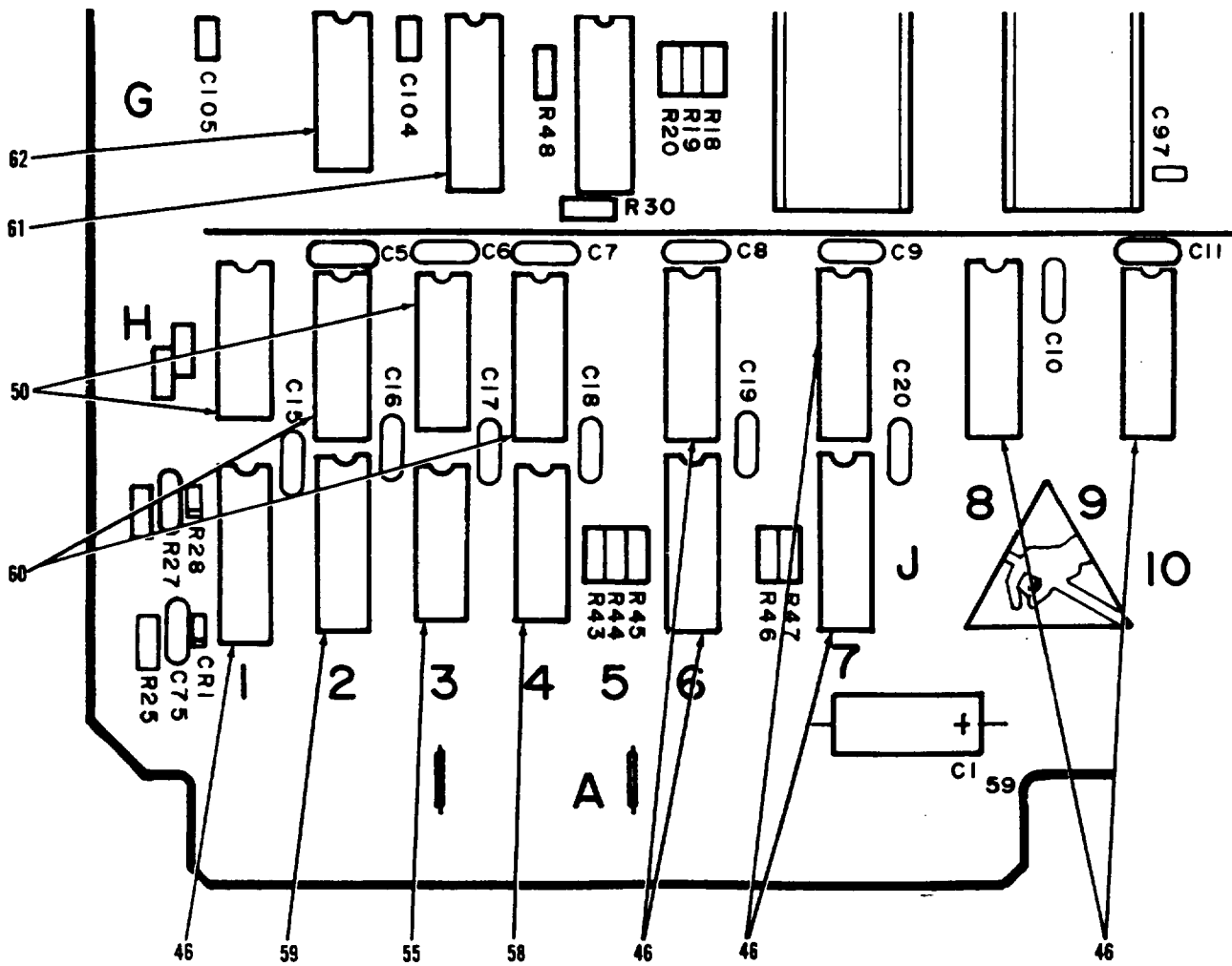
Figure 14. Circuit Card Assembly, Processor (Sheet 4 of 9)
