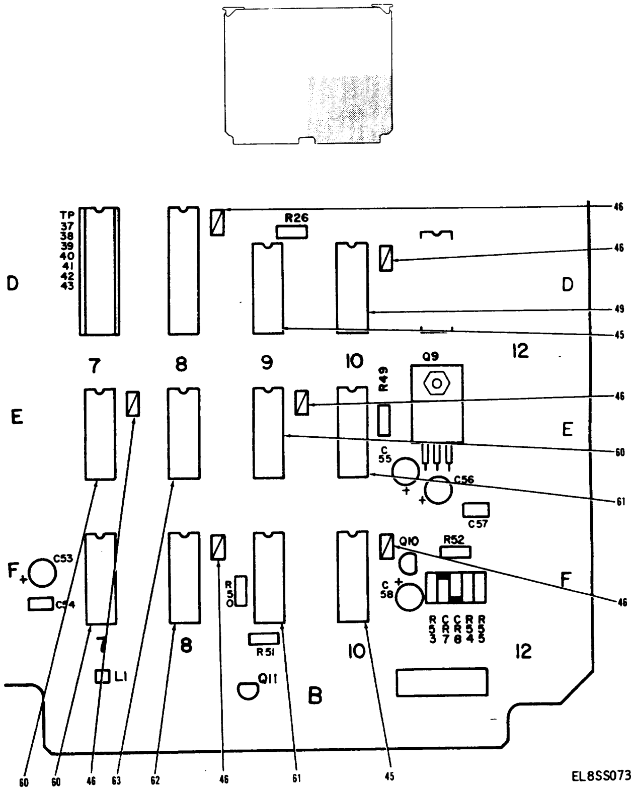
Figure 17. Circuit Card Assembly, Reference 2703 (Sheet 3 of 9)
