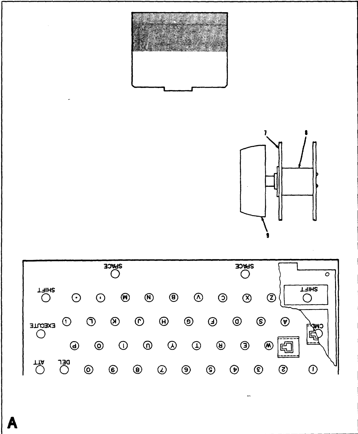
Figure 10. Circuit Card Assembly, Keyboard (Sheet 2 of 5)
